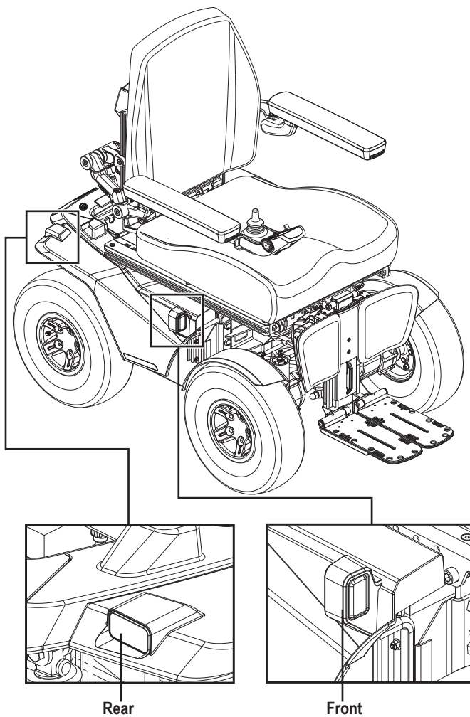
Figure 3. LED Lights
