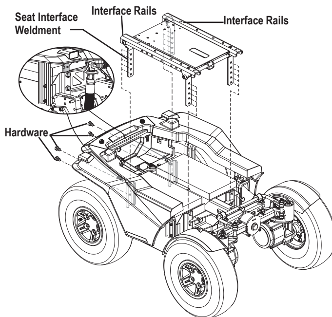
Figure 10. Seat Height/Angle Adjustment
